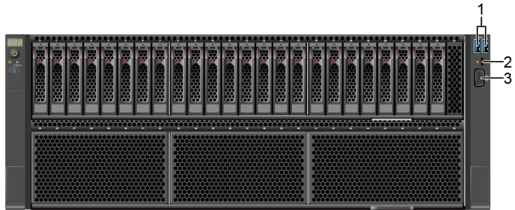
Figure 5-17 Ports on the front panel
