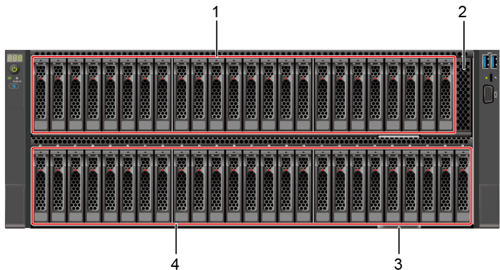
Figure 5-6 Front view
