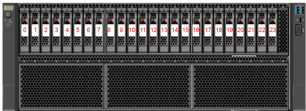
Figure 5-43 Drive numbering
