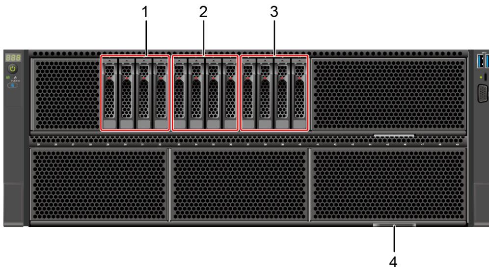
Figure 5-2 Front view
