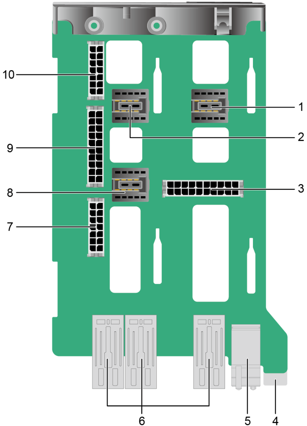
Figure 5-66 PSU backplane
