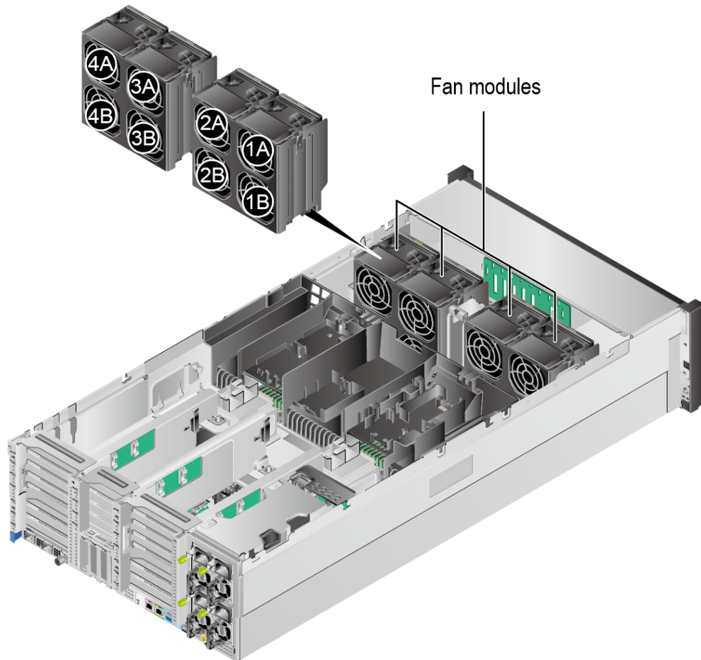
Figure 5-56 Positions of the fan modules
