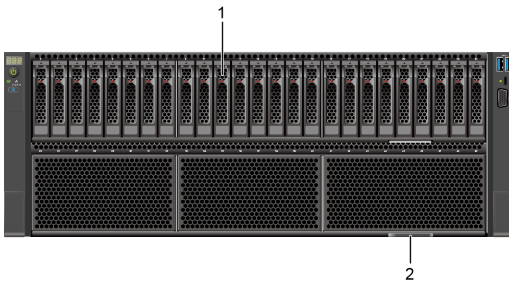
Figure 5-4 Front view
