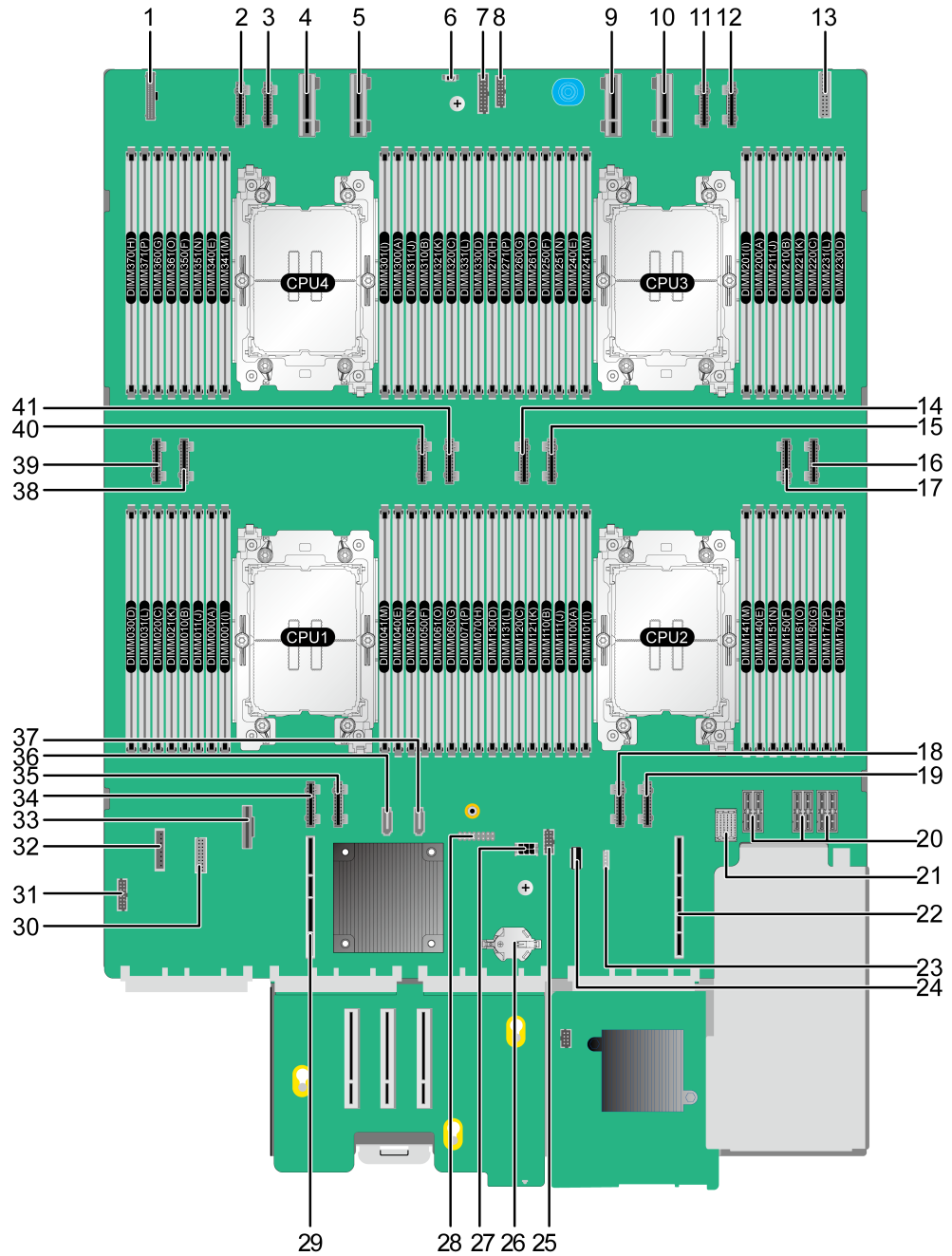
Figure 5-58 Mainboard
