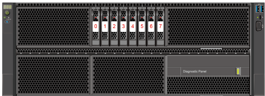
Figure 5-34 Drive Numbering
