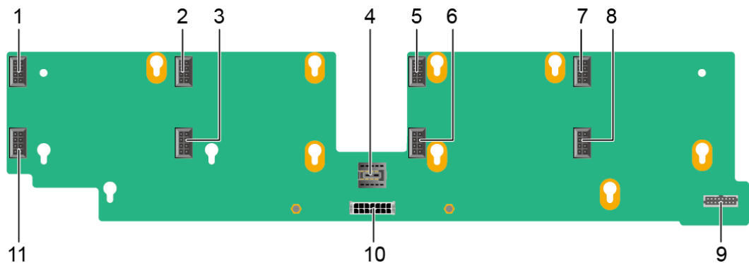
Figure 5-67 Fan board 1
