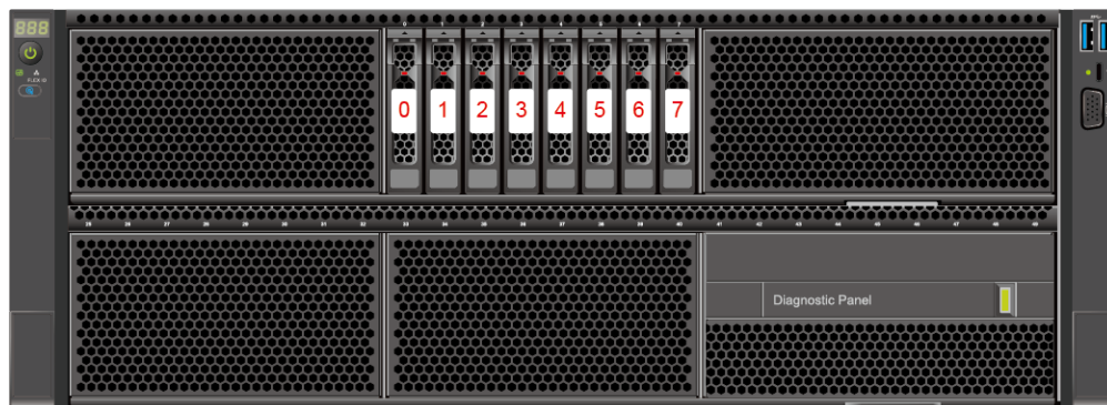
Figure 5-35 Drive Numbering
