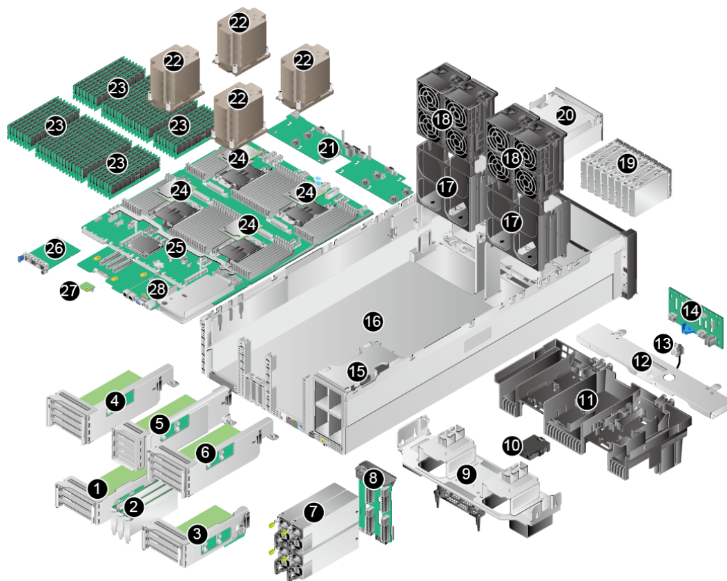
Figure 3-1 Physical structure of a server with 8 x 2.5" drives (example)
