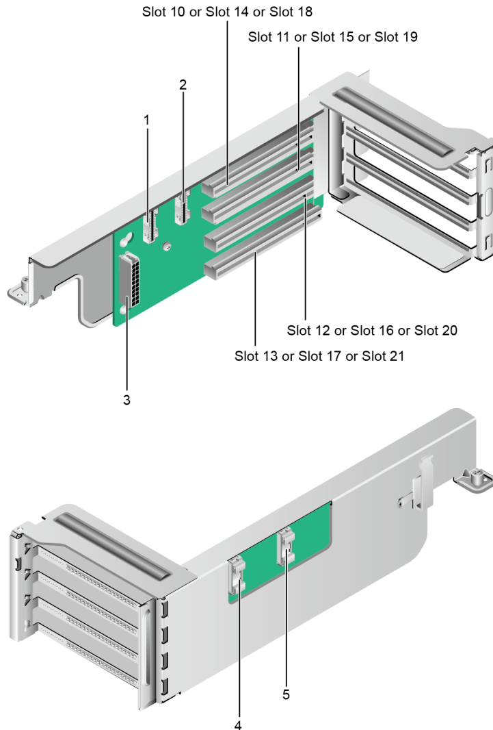
Figure 5-53 PCIe riser card 2
