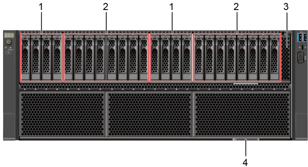
Figure 5-5 Front view
