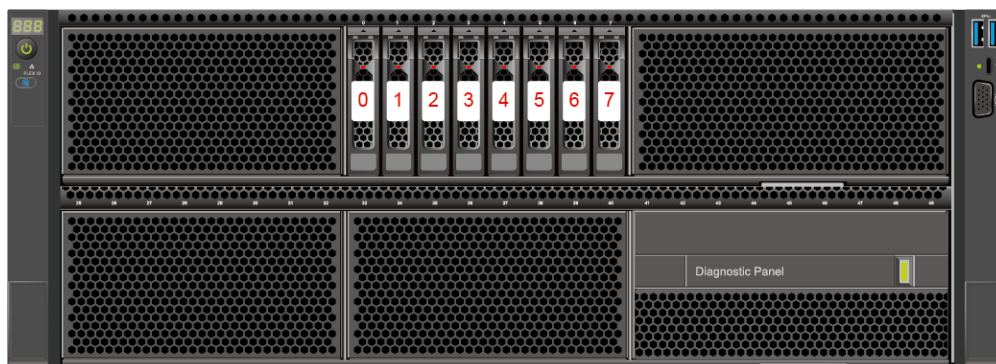
Figure 5-36 Drive numbering
