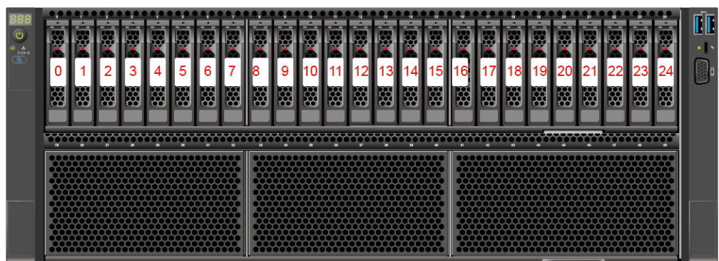
Figure 5-46 Drive numbering
