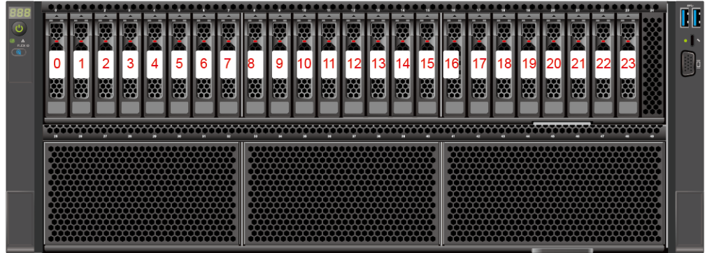
Figure 5-41 Drive numbering
