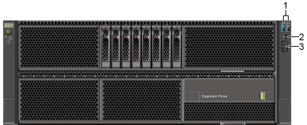
Figure 5-15 Ports on the front panel
