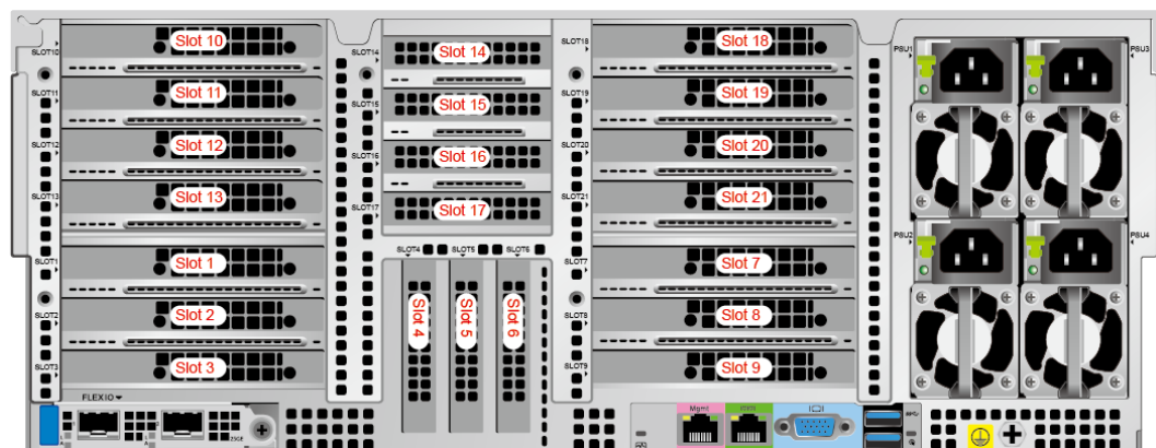
Figure 5-51 PCIe slots
