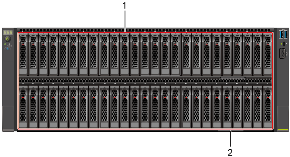
Figure 5-7 Front view
