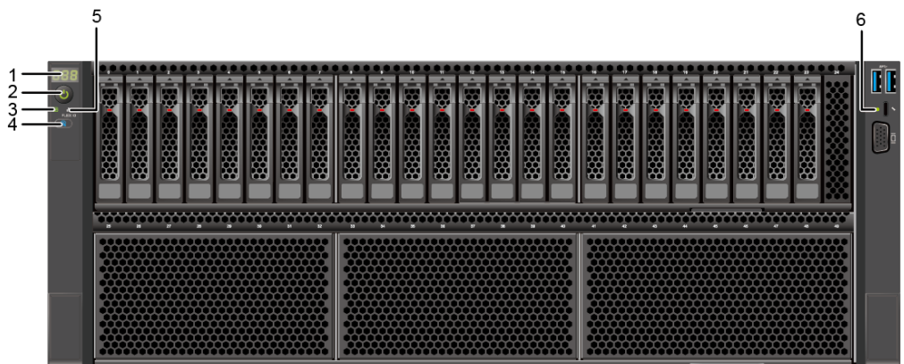
Figure 5-10 Indicators and buttons on the front panel
