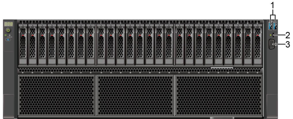
Figure 5-19 Ports on the front panel
