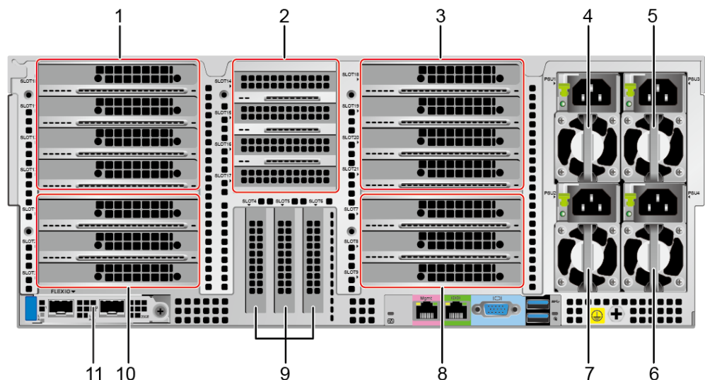
Figure 5-22 Rear view
