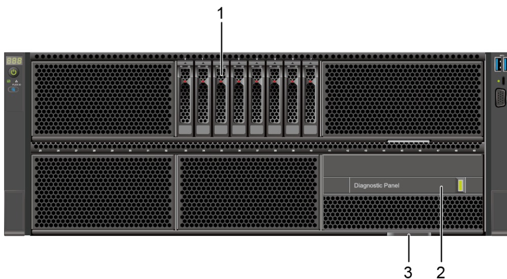
Figure 5-1 Front view
