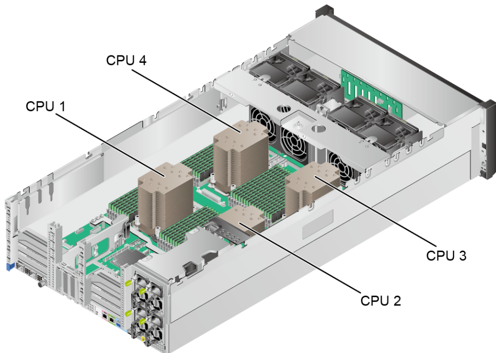
Figure 5-28 Positions of the processors
