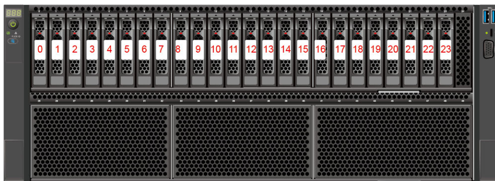
Figure 5-44 Drive numbering
