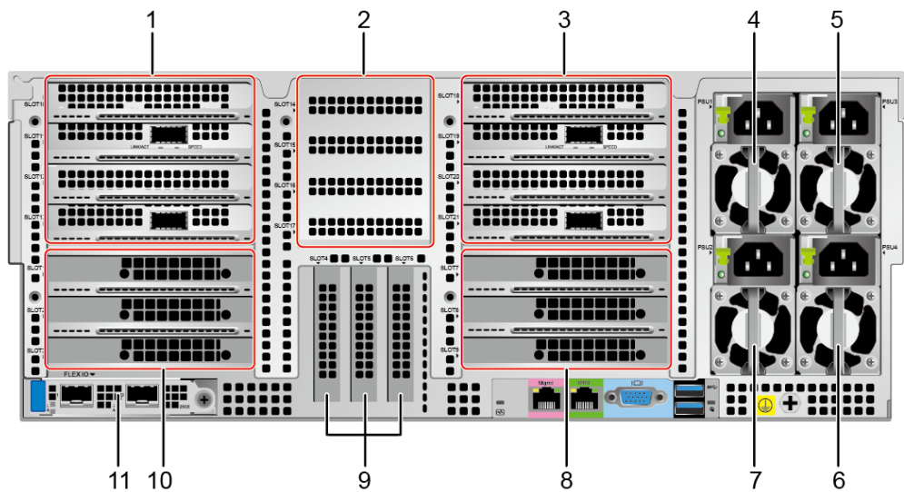
Figure 5-23 Rear view
