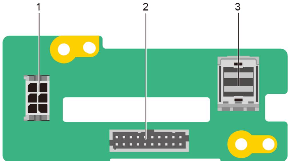
Figure 5-65 2 x 2.5" drive backplane
