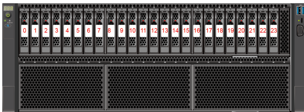
Figure 5-45 Drive numbering
