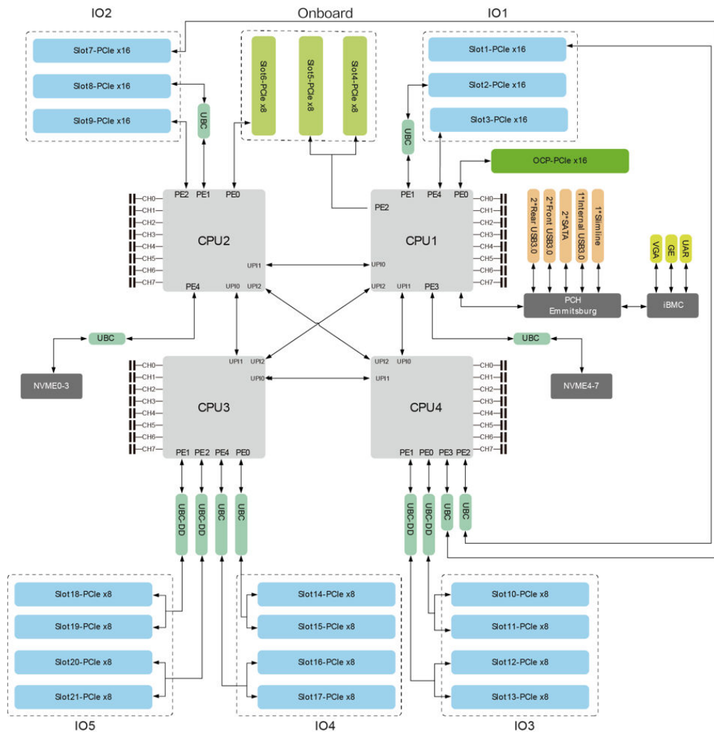
Figure 4-1 Logic structure
